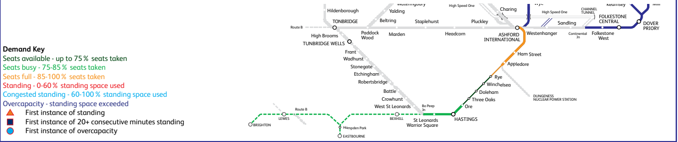
Figure 4.12E - Brighton to Ashford International capacity in 2024 (average over the whole day) - Eastbound
