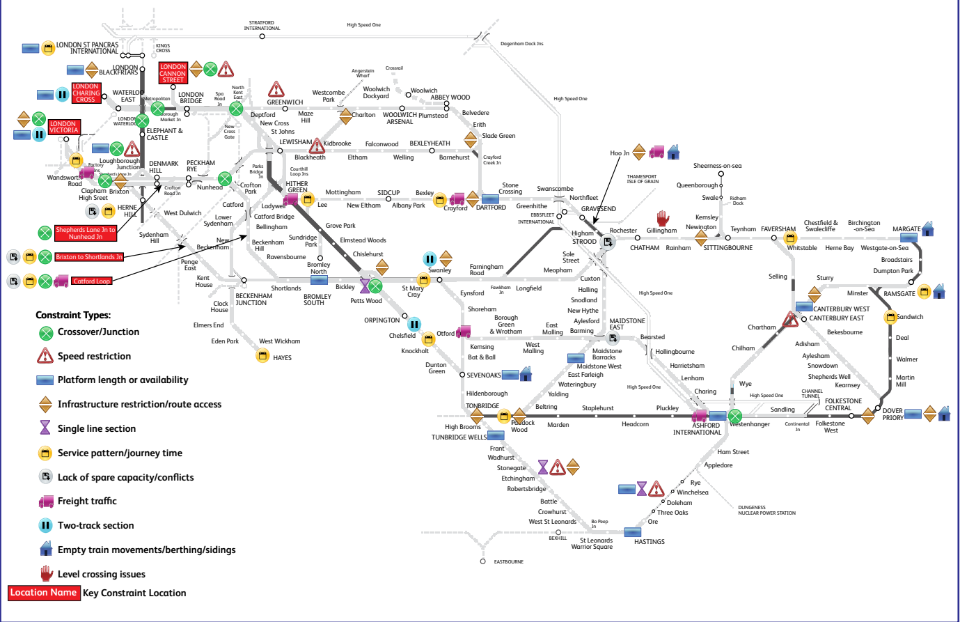
Figure 4.3 - Capability and capacity constraints
