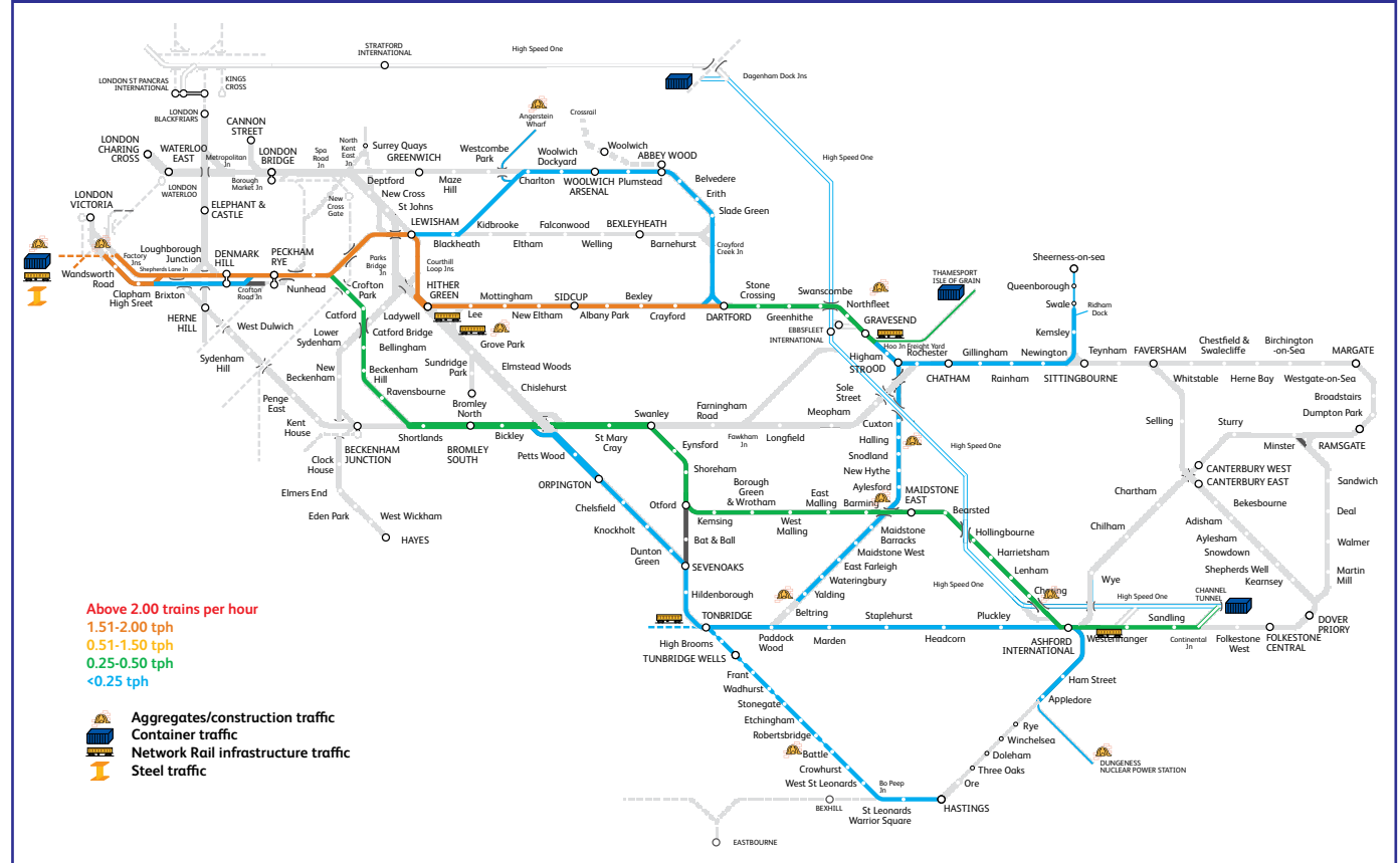
Figure 4.14 - Freight capacity requirements in 2024
