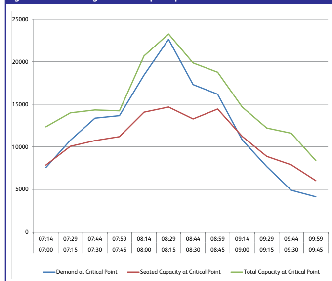
Figure 4.2 - Morning three hour peak profile
