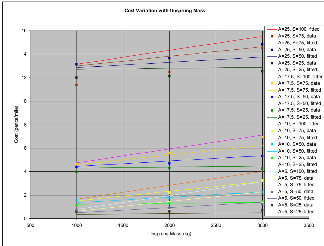
Figure 6. Relative damage variation with un-sprung mass using fitted data (hybrid formula)
