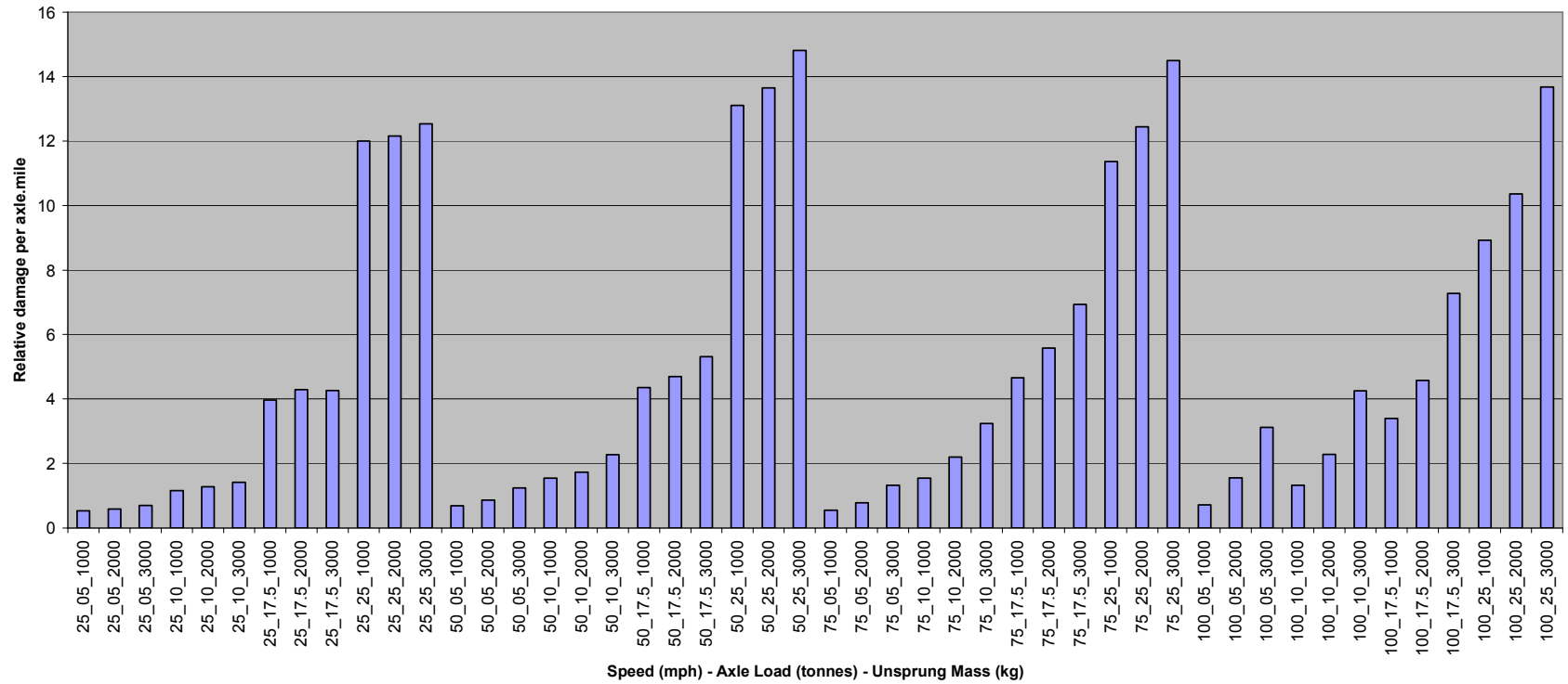
Figure 3. VTISM-derived relative damage indices for variant cases
