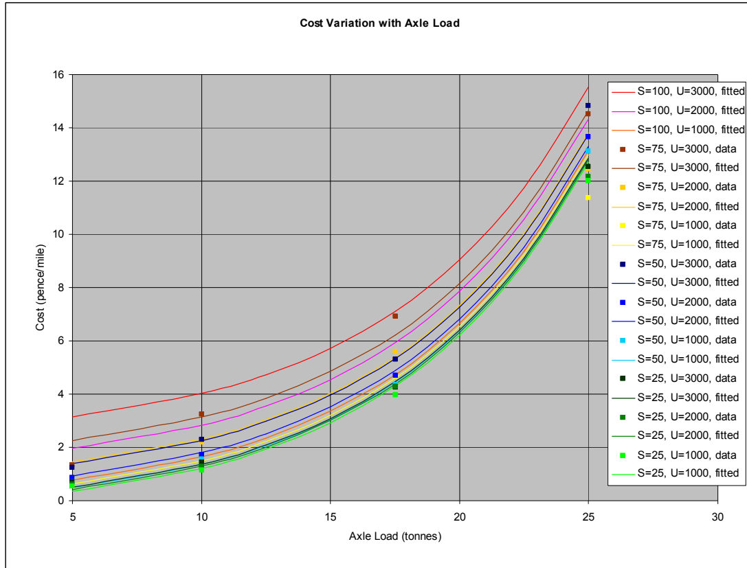
Figure 5. Relative damage variation with axle load using fitted data (hybrid formula)
